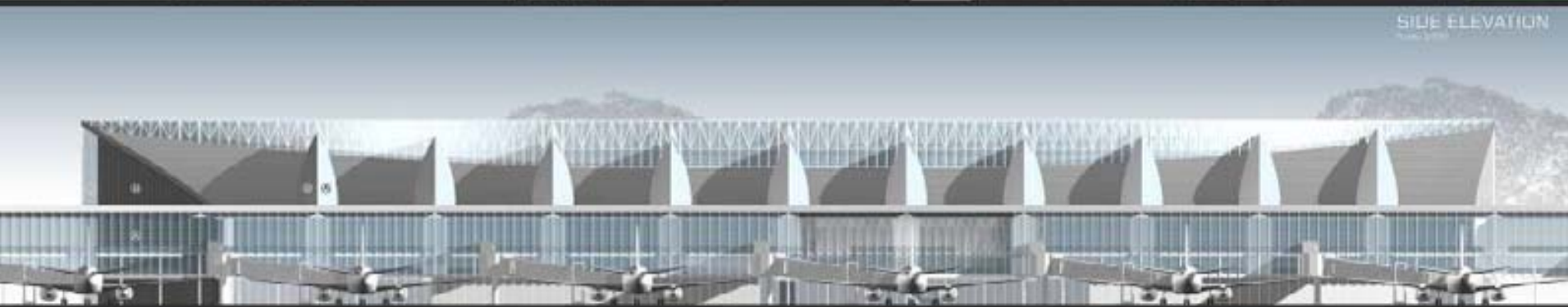
AIRSIDE ELEVATION Scale 1/200
